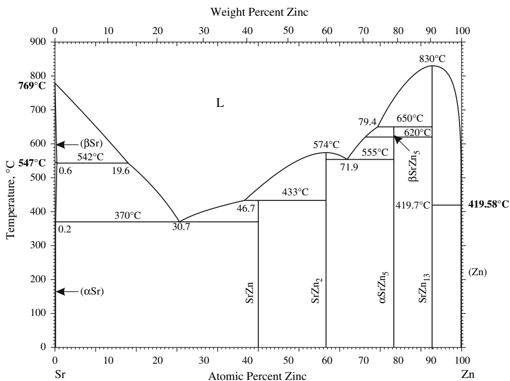
Fig. 1 Sr-Zn phase diagram
